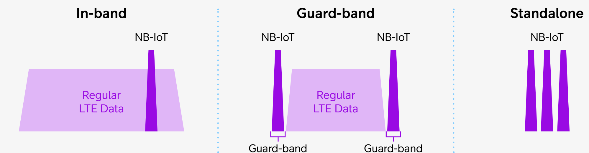
FIGURE 2: NB-IOT DEPLOYMENT MODES
